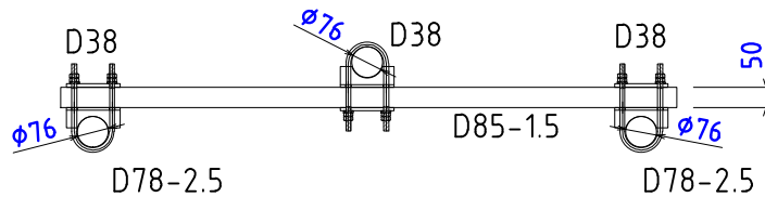
Parallel frame for 5G antennas-2.5m/1.0m
