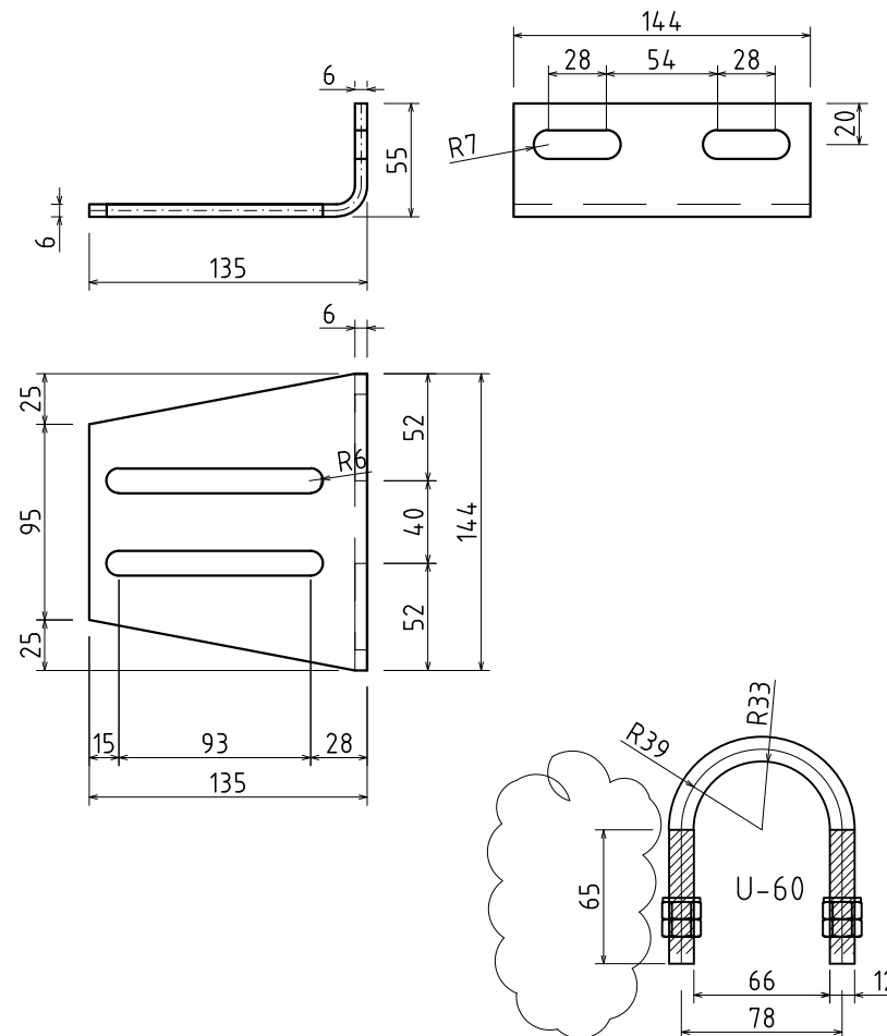
ANTENNA BRACKET AND BENDED RRU-BRACKET ON ANGLED LEGS
