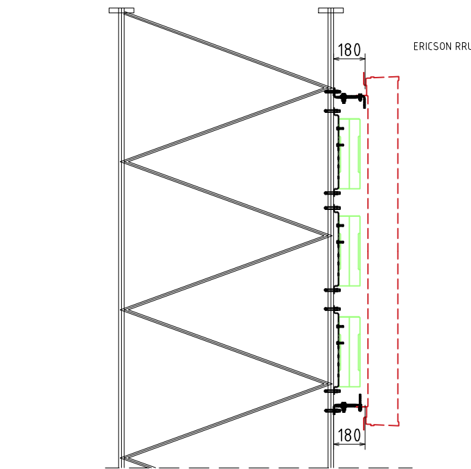
ANTENNA BRACKET AND FLAT RRU-BRACKET ON BENDED LEGS
