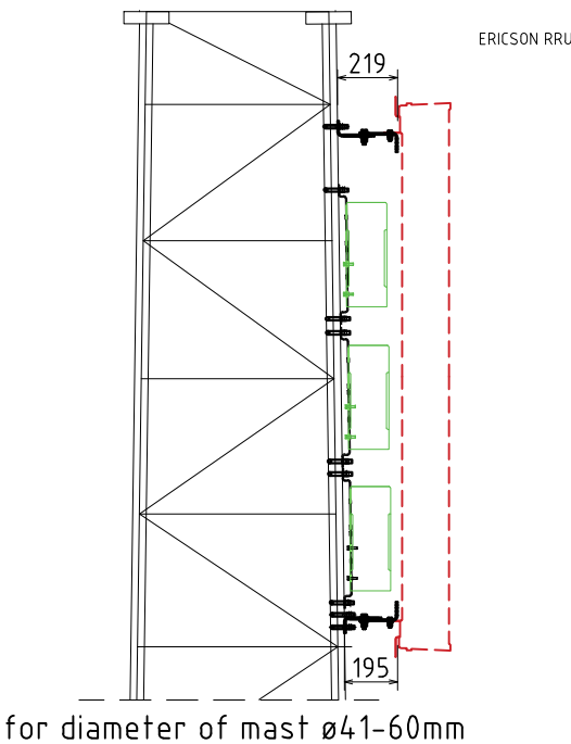
ANTENNA BRACKET AND BENDED RRU-BRACKET ON ANGLED LEGS
